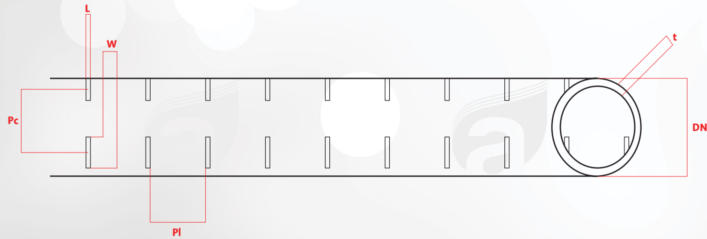
Draw 2: Vertical Slotted
